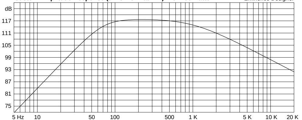
Custom Amplitude Response (dB-SPL/Hz at 1 m) with 150 watts
