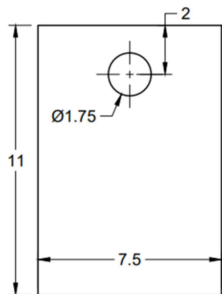
1 x Back
